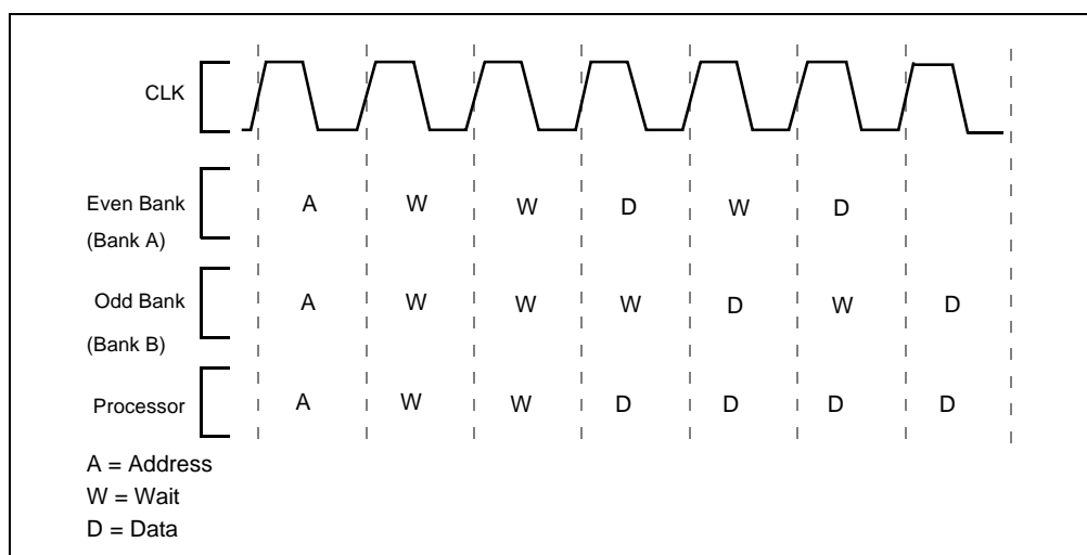
Figure 4-3. Two-way Interleaving
