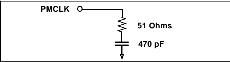
Figure 5-10. Squall II Module Clock Termination
